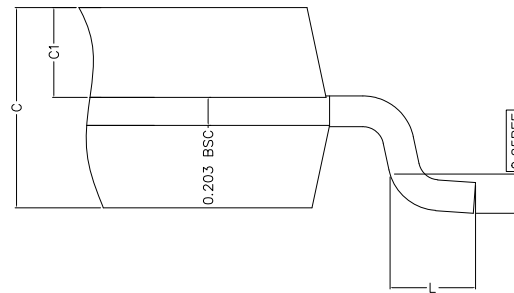
DETAIL I
